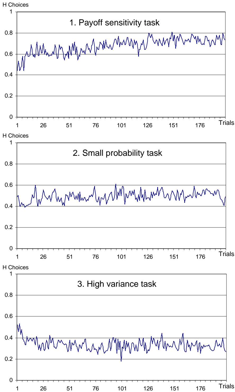
Figure 2: Proportion of choices from the High expected value alternative (H) as a function of time in the three experimental tasks of study 1.
