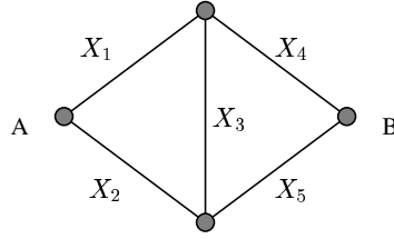
Figure 1: Stochastic shortest path from A to B
